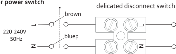
Picture 1. Dryer with timer power switch
